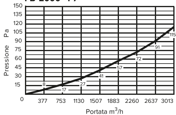
FB 2000 - F7
