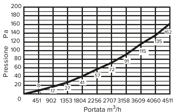
FB 2500/3000 F7
