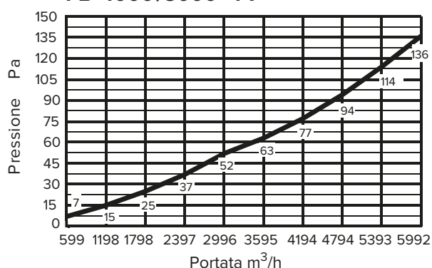
FB 4000/5000 - F7
