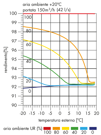
EFFICIENCY IN ACCORDANCE WITH CONDENSATION HEAT
